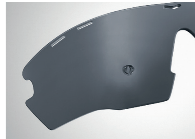
Dent in test lens after undergoing an impact test – the steel ball does not pass through the lens.
